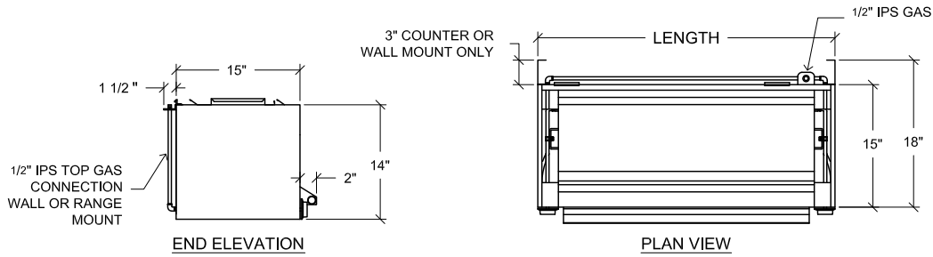
MODEL QCM-36 SHOWN
