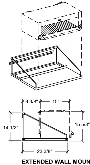
EXTENDED WALL MOUNT
